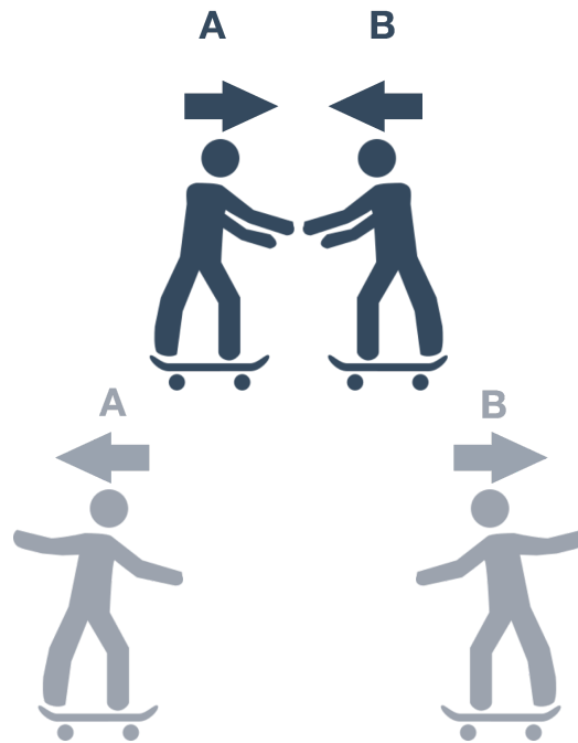
Figure 1: When two people on skateboards "push" on one another (action) they will move in the opposite direction (reaction).
