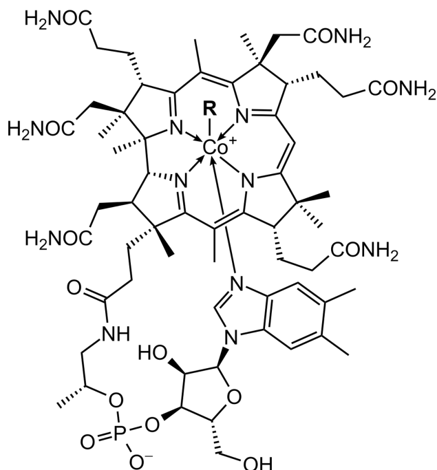
Figure 6: Structural Formula (ie., little chemical pictures). Shown: "Skeletal structural formula of Vitamin B12. Many organic molecules are too complicated to be specified by a chemical formula (molecular formula) [31]."
