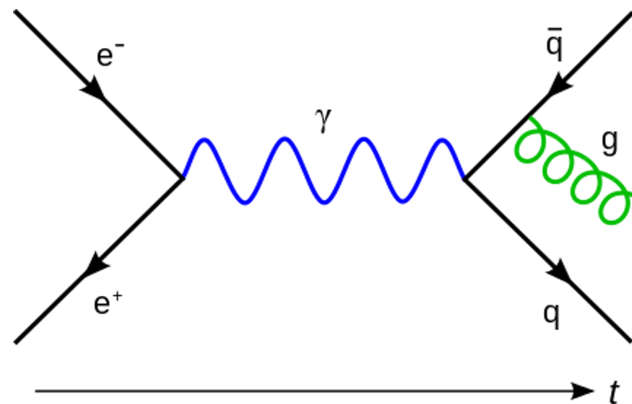
Figure 5: Feynman diagram, shown: "an electron ( e^- ) and a positron ( e^+ ) annihilate, producing a photon ( \gamma , represented by the blue sine wave) that becomes a quark–antiquark pair (quark q , antiquark \bar{q} ), after which the antiquark radiates a gluon ( g ), represented by the green helix)."
